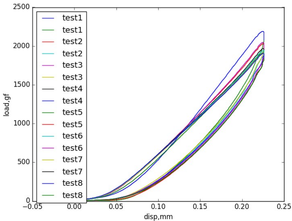
Repeatability of ramp load -unload before preconditioning
