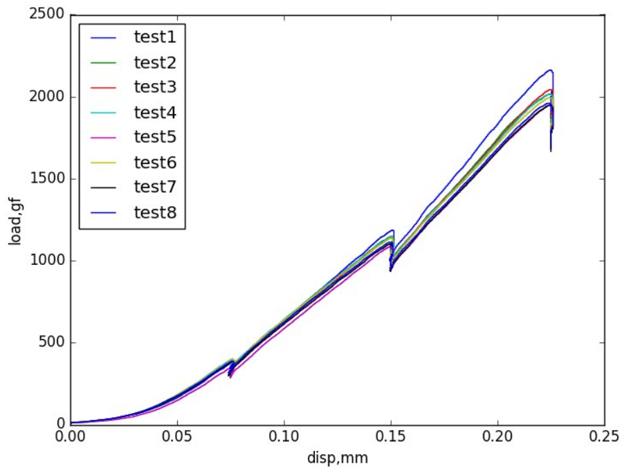
Stress-relaxation repeatability
