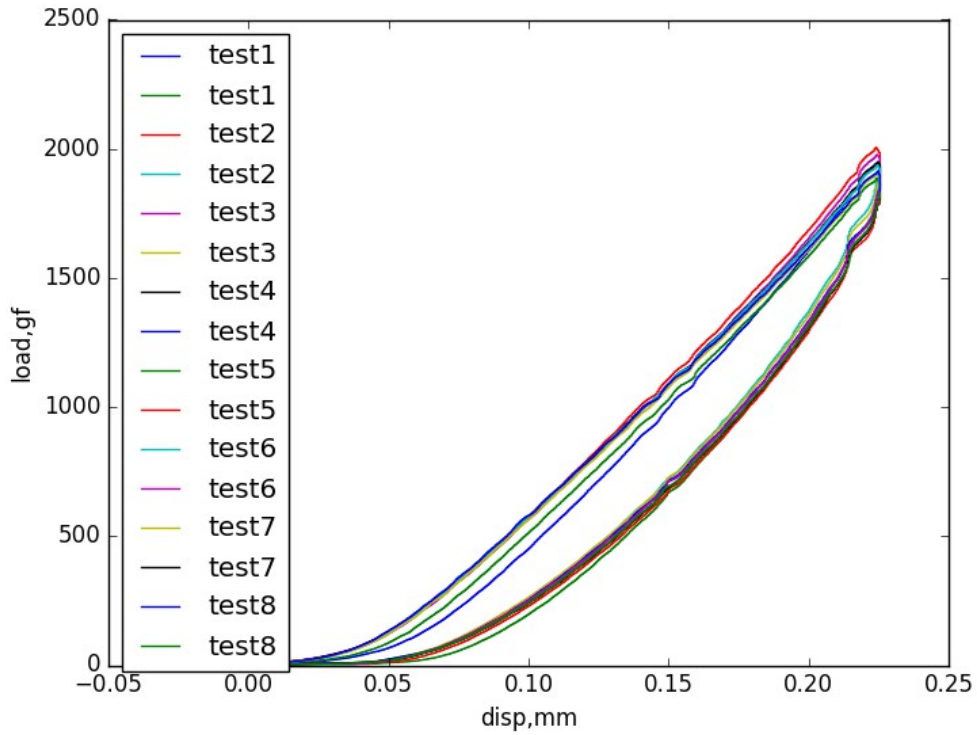
Repeatability of ramp load-unload after preconditioning
