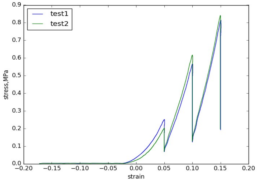
Unconfined compression
