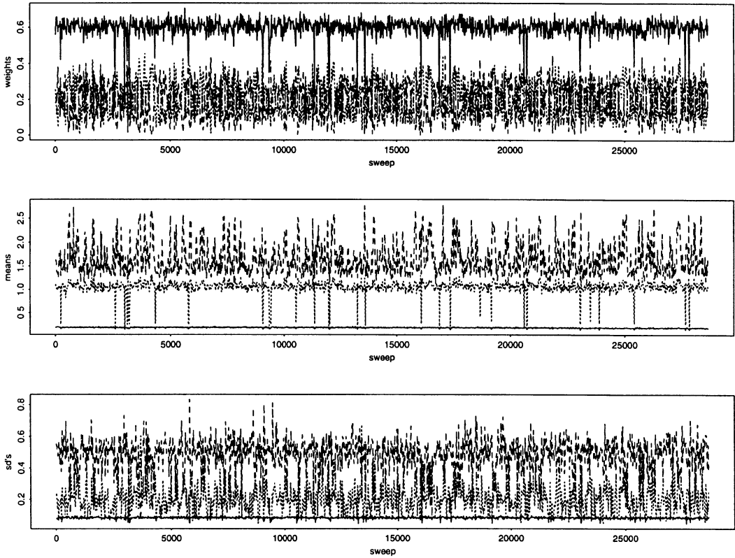
Fig. 8. Traces of parameter estimates against visits to k = 3 , enzyme data
