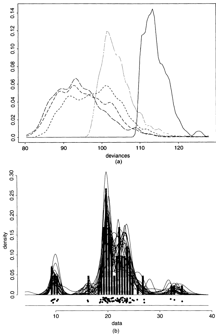
Fig. 3. (a) Posterior distributions of deviances for the enzyme data (—, k = 2 ; ·····, k = 3 ; - - -, k = 4 ; - · - ·, k = 5 ; — — —, k = 6 ); (b) sample from the posterior distribution of f(\cdot|k, w, \theta) for the galaxy data
