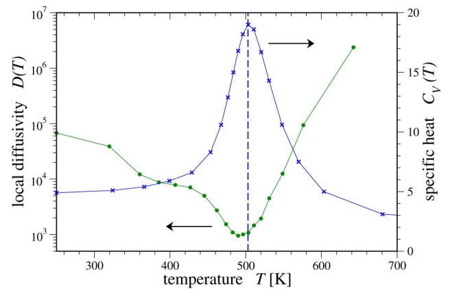
FIG. 3. Local diffusivity D(T) (left ordinate) for a random walk in temperature space performed by a replica in a parallel tempering simulation of the chicken villin headpiece subdomain HP-36 using the ECEPP/2 force field and an implicit solvent. The diffusivity shows a strong modulation with temperature; note the logarithmic scale of the left ordinate. A pronounced minimum in the local diffusivity occurs slightly below the helix-coil transition around T \approx 500 K where the specific heat C_v(T) (right ordinate) has a maximum (dashed line).
